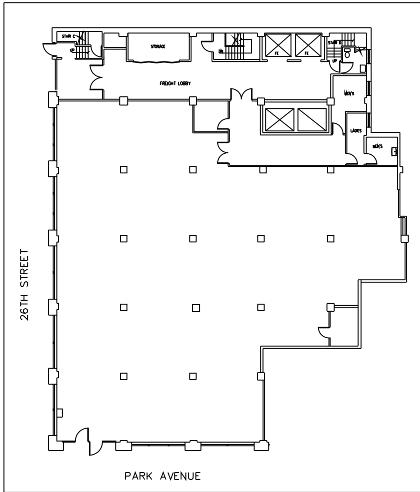
PART GROUND FLOOR
